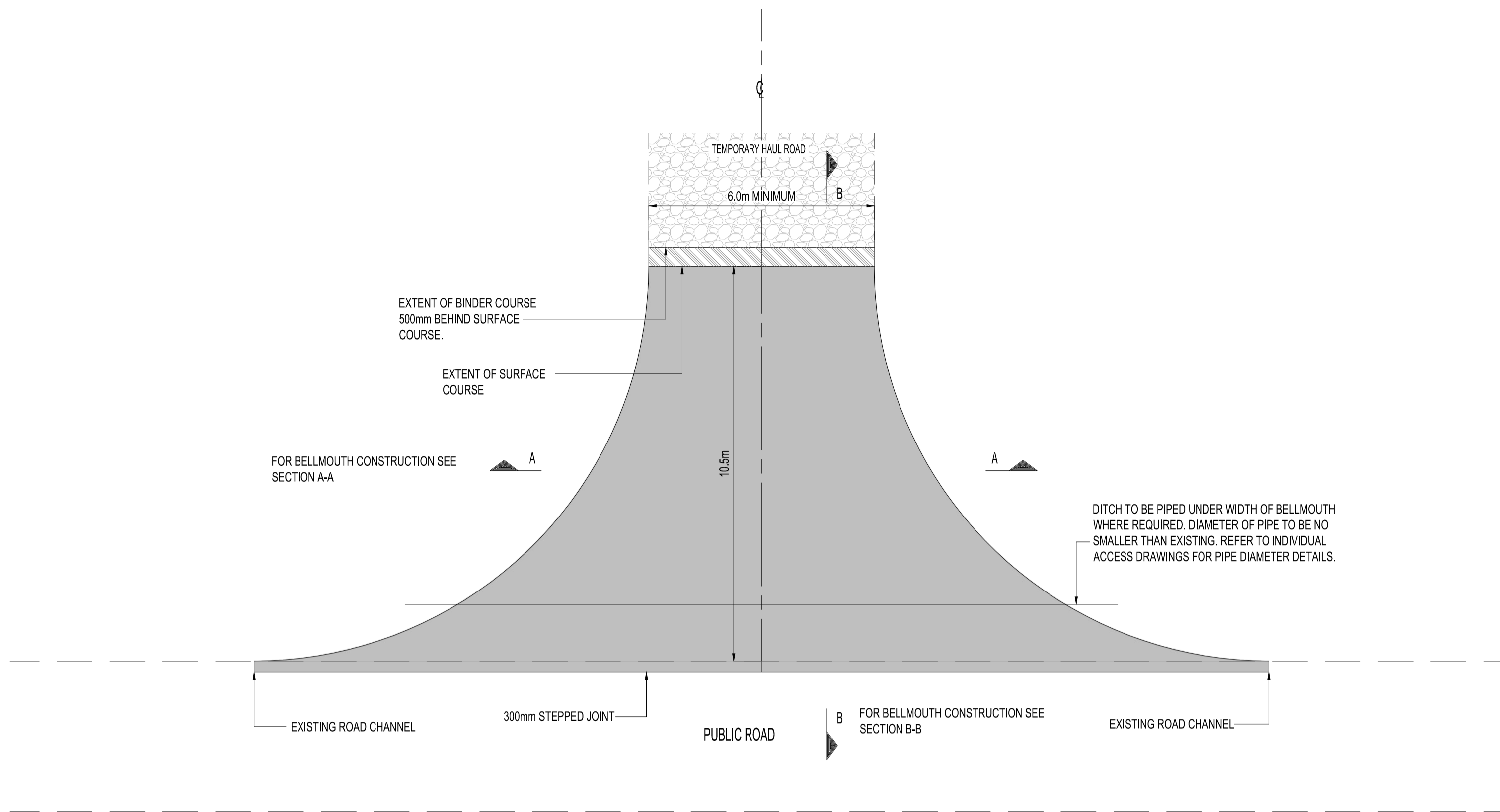
PROPOSED ACCESS BELLMOUTH (SCALE 1:100)
